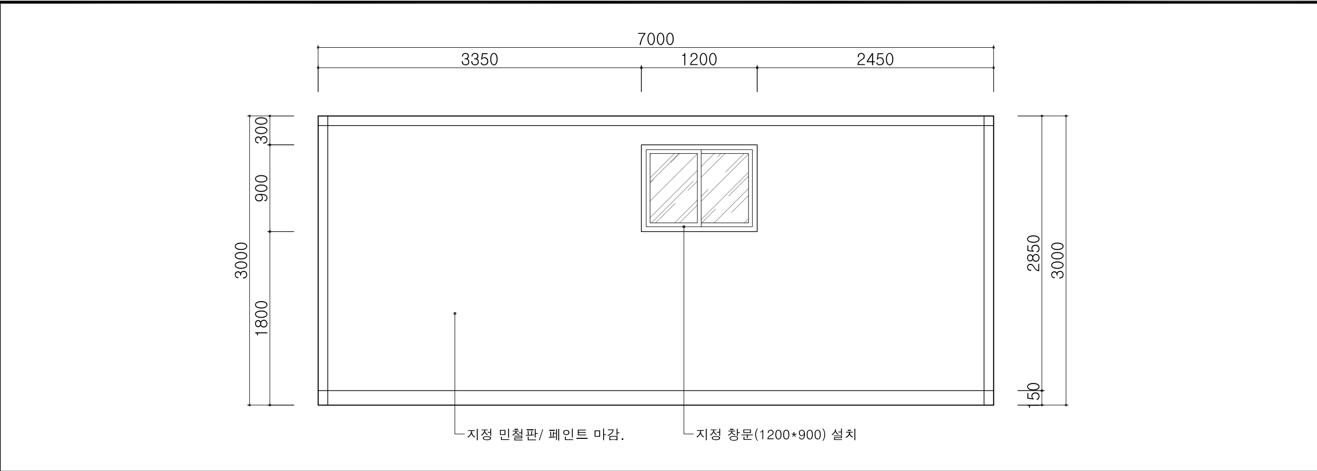
ELEVATION 'A'
